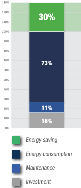
LIFE CYCLE COST SAVINGS IN 5 YEARS OF A NOBEL V, COMPARED TO A FIXED SPEED COMPRESSOR WITH THE SAME POWER
